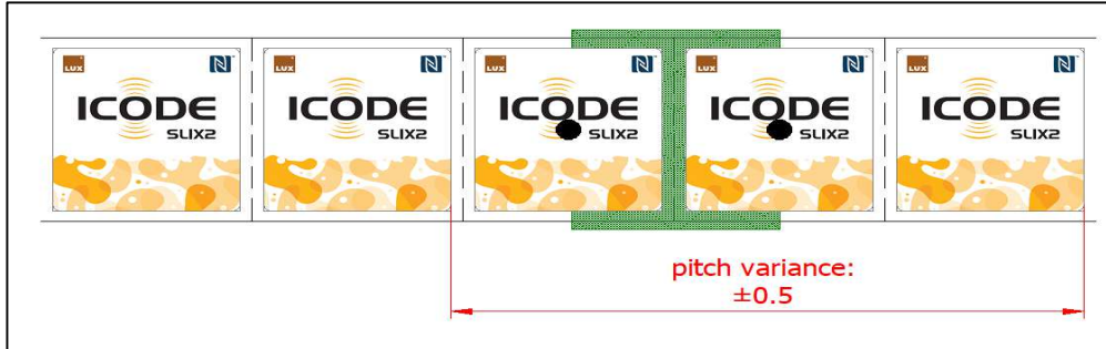
Figure 4: Pitch tolerance at splicing positions
